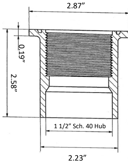
Hub Adapter
