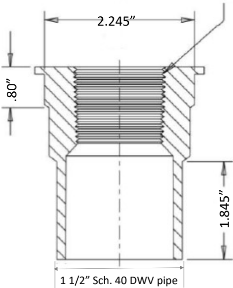
Spigot Adapter
